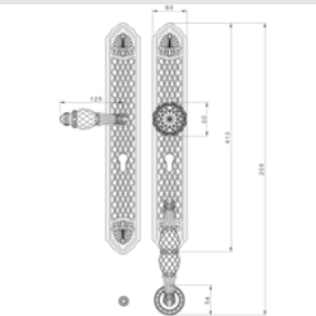
0J3007.SZ85.** 0J3007.SNZ85.** Entrance door set with fixed knob and keyhole europrofile 85mm
