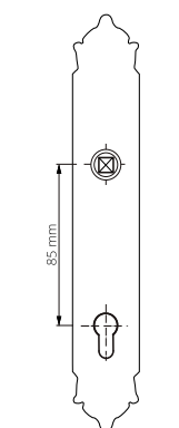
85Y EUROPROFILE KEY HOLE
