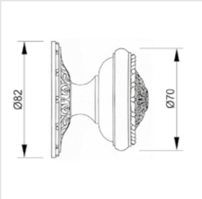
OC3616.000.** Door fixed knob
