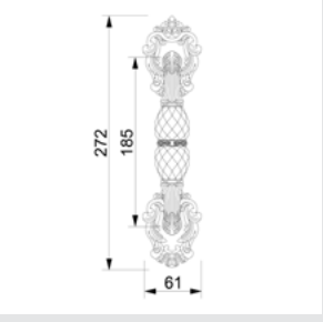
0N7405.S00.** 0N7405.SN0.** Door pull handle on roses with Swarovski crystal
